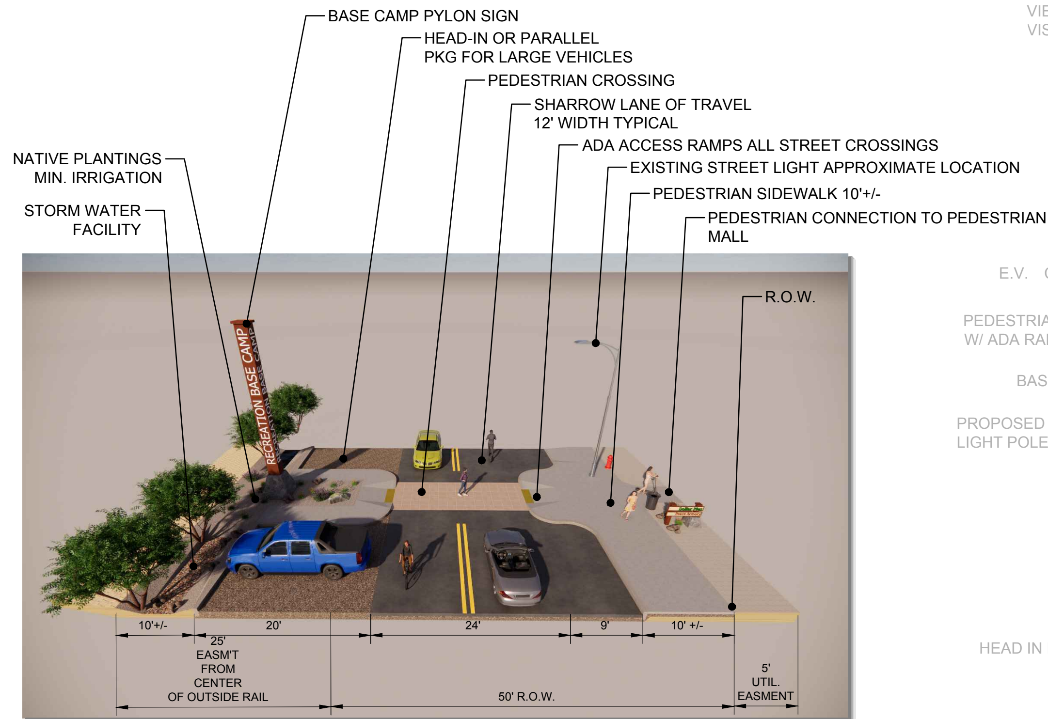
COMMERCIAL STREET CROSS SECTION
